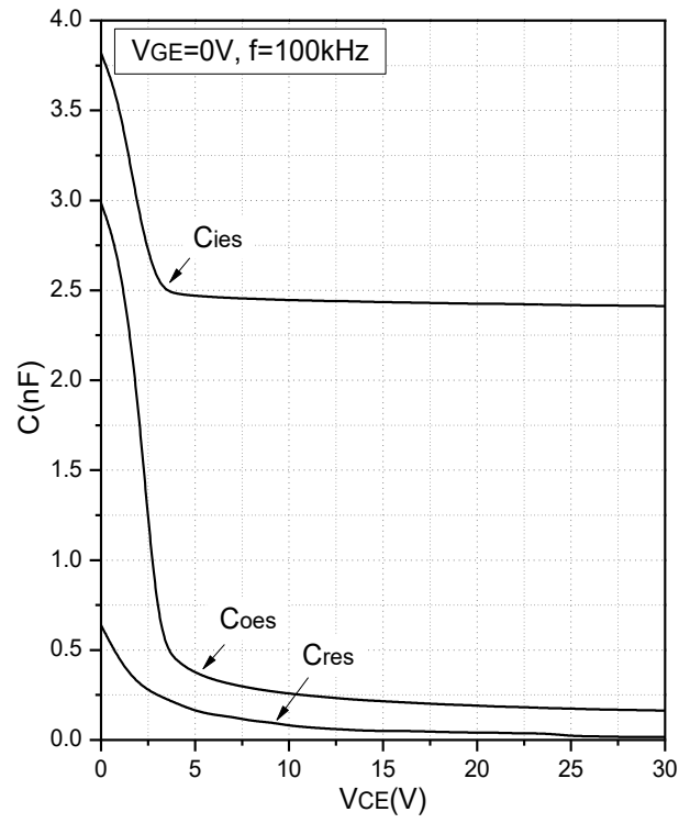
Fig.12 Capacitance Characteristics
