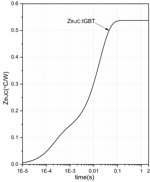
Fig.9 Transient Thermal Impedance IGBT(Inverter)
