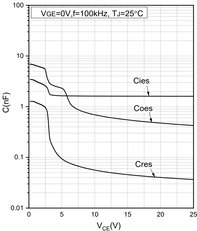
Fig.11 Capacitance Characteristics(Inverter)
