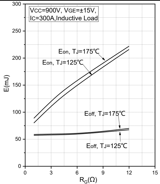
Fig.6 Typical Switching Loss IGBT vs. Gate Resistance
