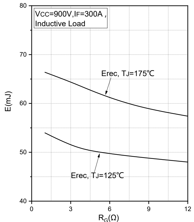
Fig.8 Typical Switching Loss Diode vs. Gate Resistance
