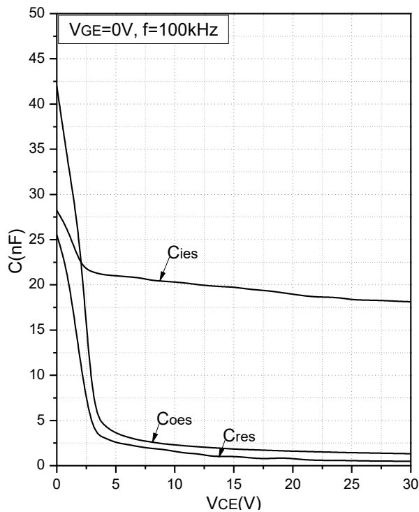
Fig.11 Capacitance Characteristics
