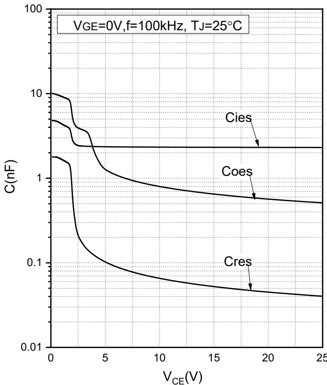
Fig.11 Capacitance Characteristics
