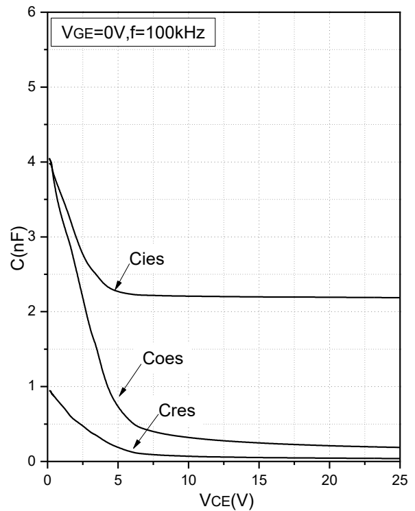
Fig.12 Capacitance Characteristics
