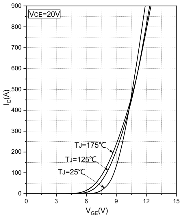
Fig.3 Transfer Characteristic
