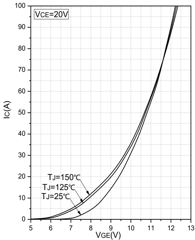
Fig.3 Transfer Characteristic
