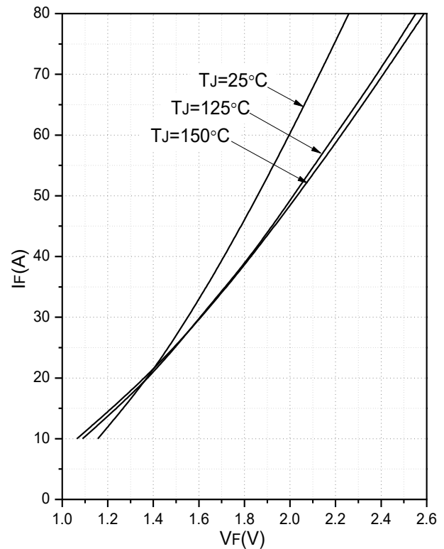
Fig.4 Forward Characteristics of Diode
