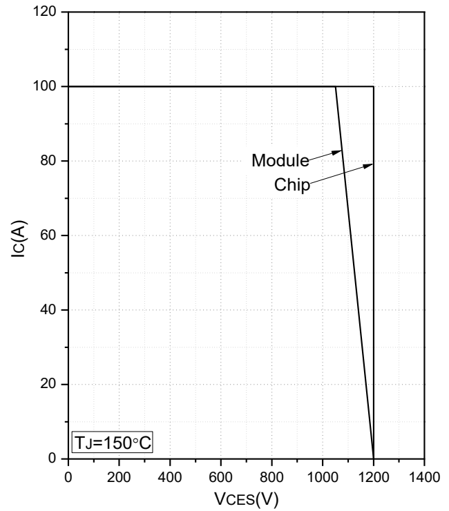
Fig.10 Reverse Bias Safe Operation Area
