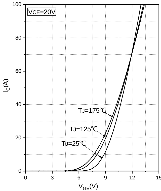
Fig.3 Transfer Characteristic(Inverter)
