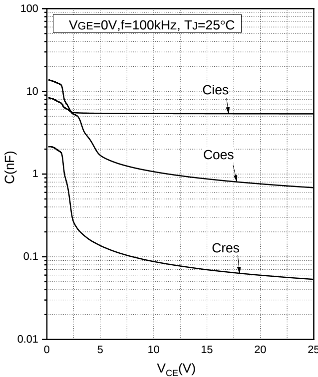
Fig.11 Capacitance Characteristics(Inverter)
