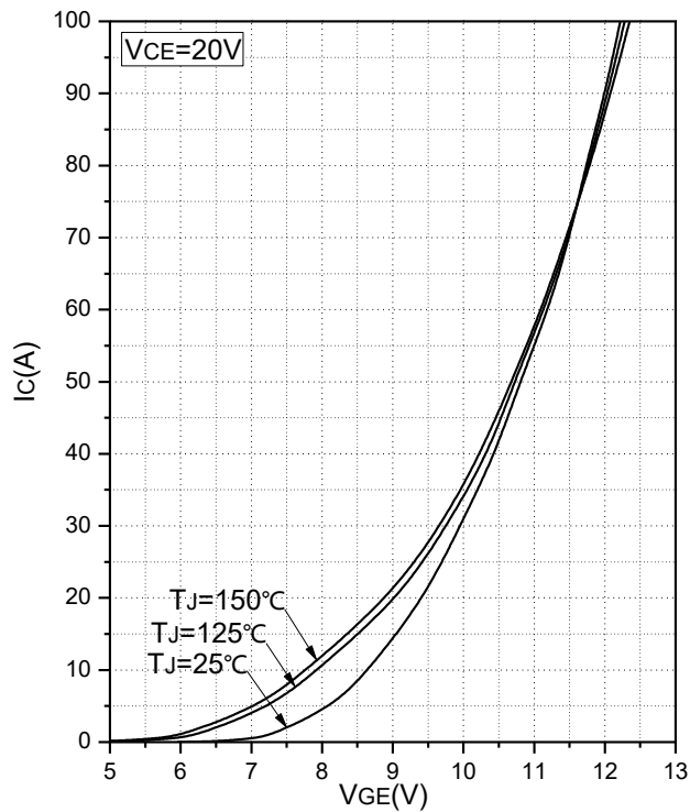
Fig.3 Transfer Characteristics(Inverter)
