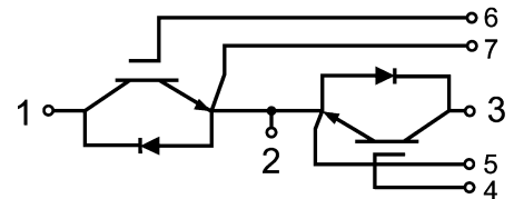
Circuit Diagram
