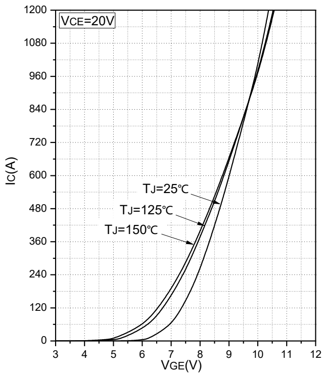
Fig.3 Transfer Characteristics
