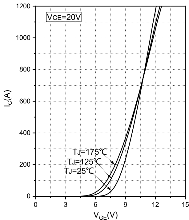
Fig.3 Transfer Characteristic
