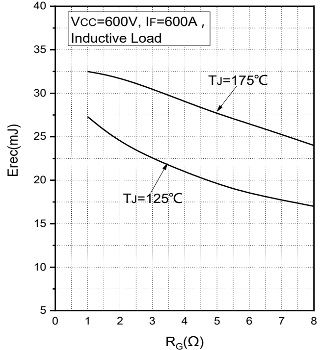
Fig.8 Typical Switching Loss vs. Gate Resistance
