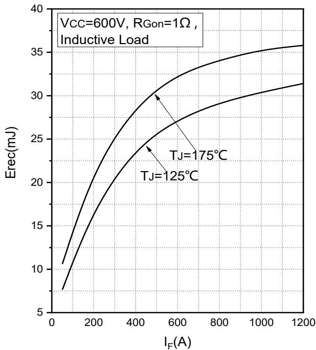
Fig.7 Typical Switching Loss vs. Forward Current
