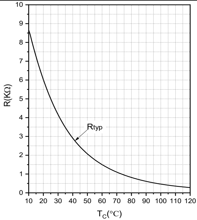
Fig.13 NTC Temperature Characteristics
