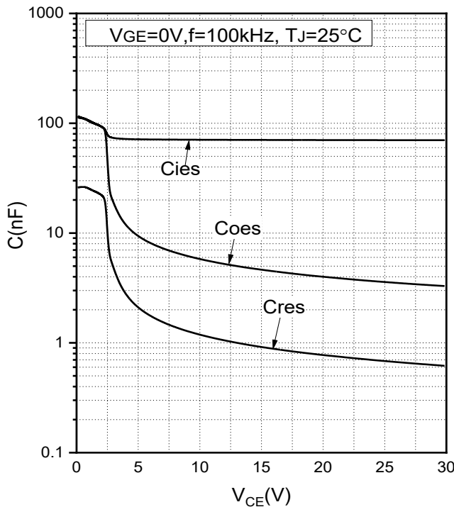
Fig.11 Capacitance Characteristics
