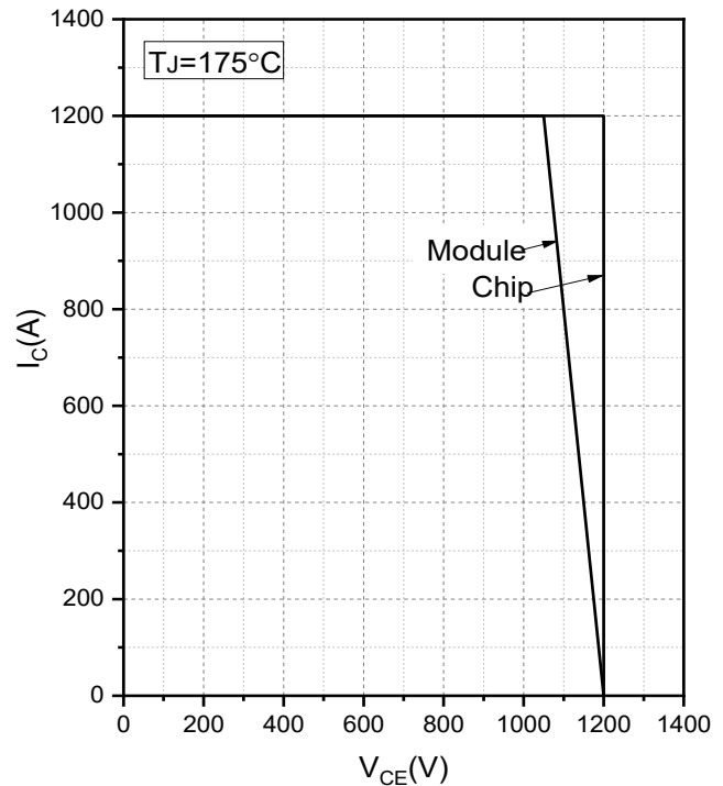
Fig.12 Reverse Bias Safe Operation Area (RBSOA)
