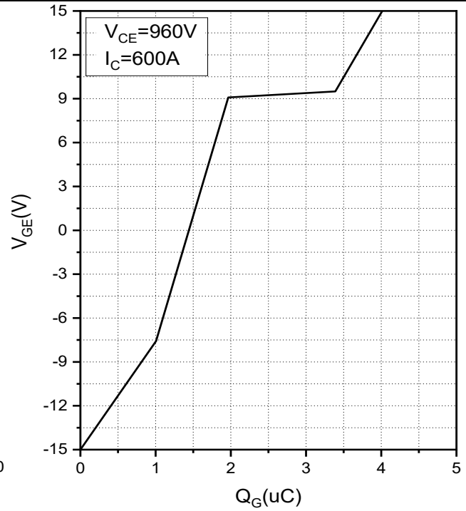
Fig.14 Gate Charge Characteristics
