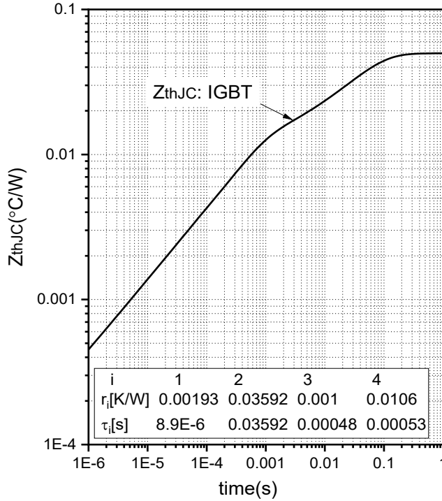
Fig.9 Transient Thermal Impedance (IGBT)
