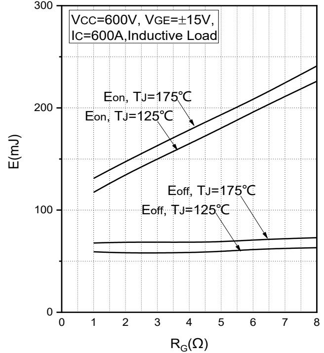
Fig.6 Typical Switching Loss vs. Gate Resistance
