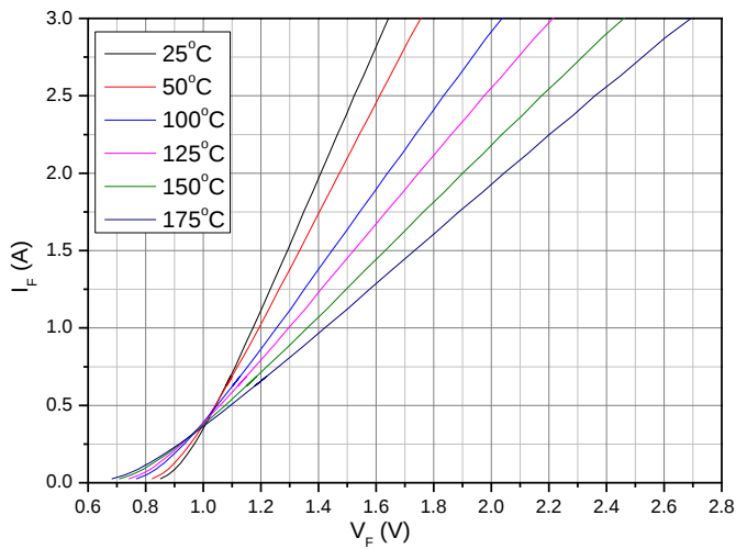
Figure 1. Forward Characteristics
