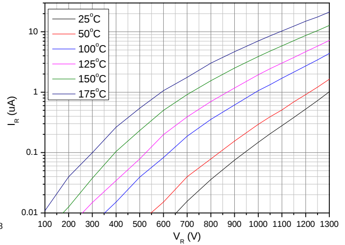
Figure 2. Reverse Characteristics
