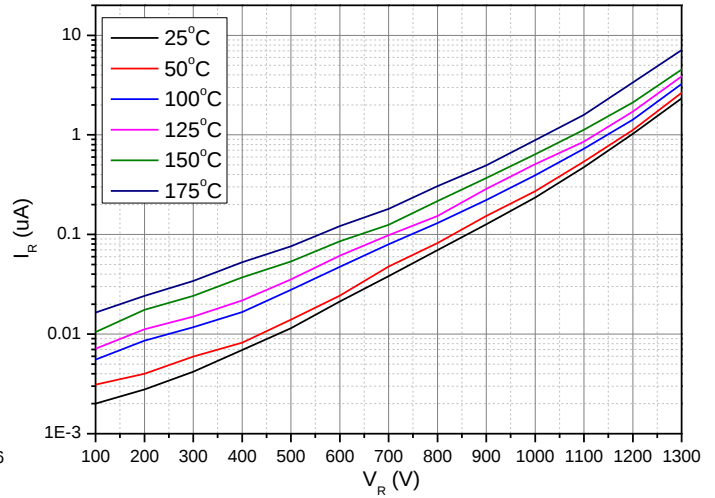
Figure 2. Reverse Characteristics
