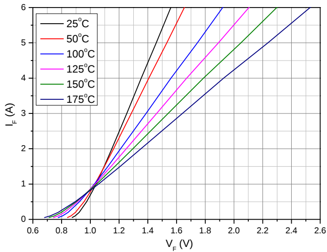
Figure 1. Forward Characteristics
