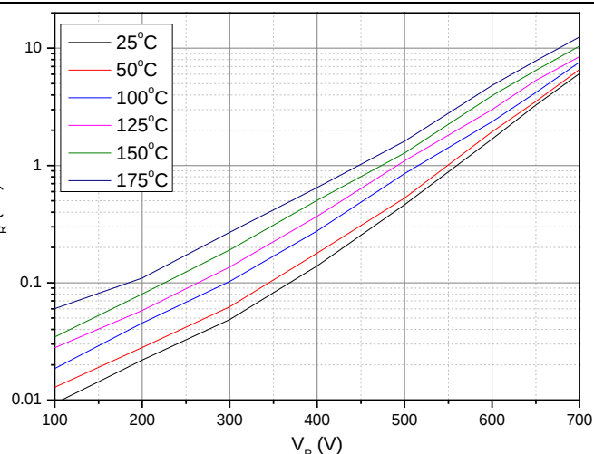
Figure 2. Reverse Characteristics
