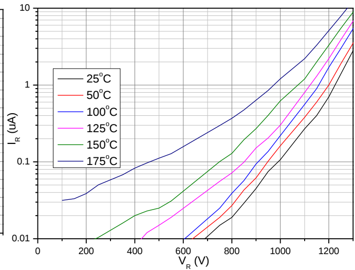
Figure 2. Reverse Characteristics
