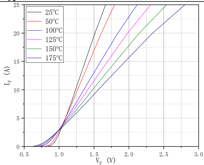
Figure 1. Forward Characteristics
