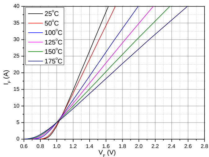
Figure 1. Forward Characteristics
