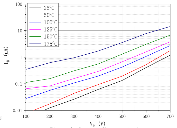
Figure 2. Reverse Characteristics
