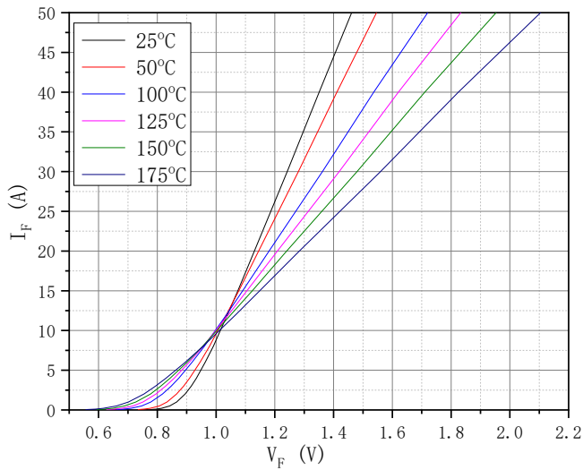
Figure 1. Forward Characteristics
