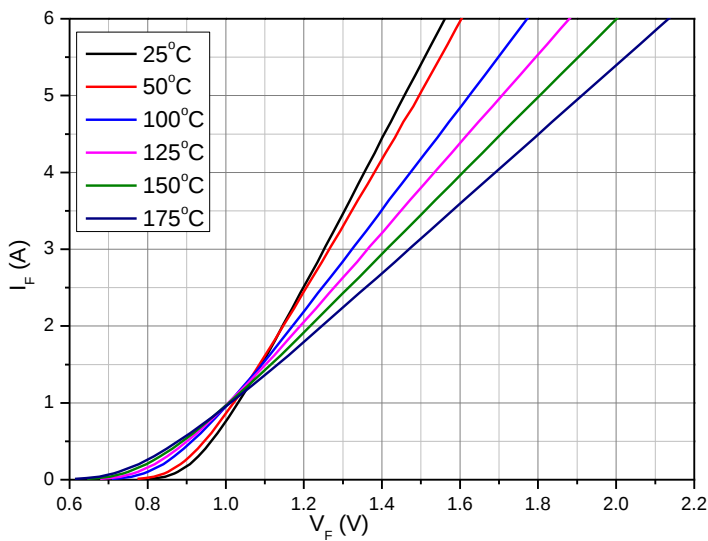
Figure 1. Forward Characteristics
