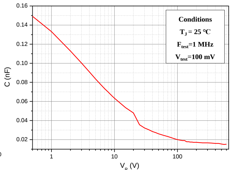
Figure 4. Capacitance vs. Reverse Voltage
