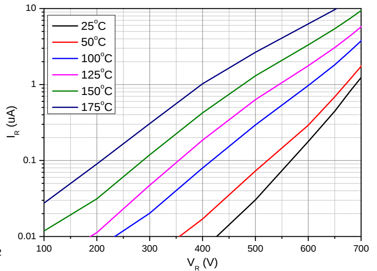
Figure 2. Reverse Characteristics
