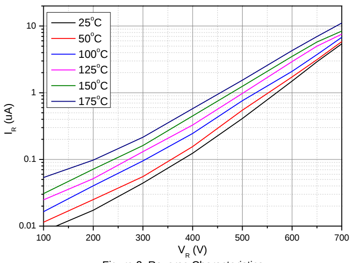
Figure 2. Reverse Characteristics
