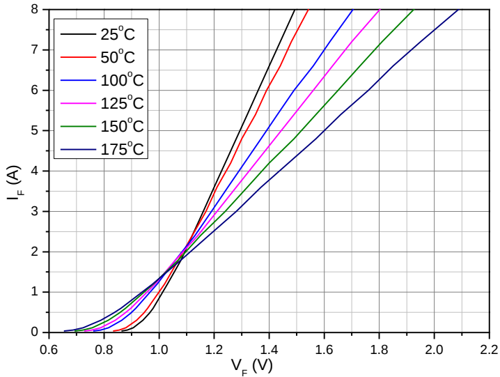
Figure 1. Forward Characteristics
