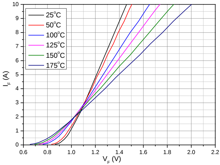
Figure 1. Forward Characteristics
