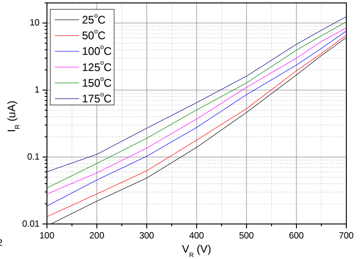
Figure 2. Reverse Characteristics
