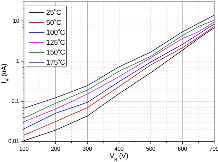
Figure 2. Reverse Characteristics
