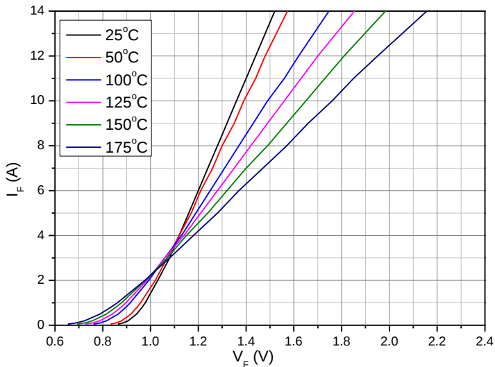
Figure 1. Forward Characteristics
