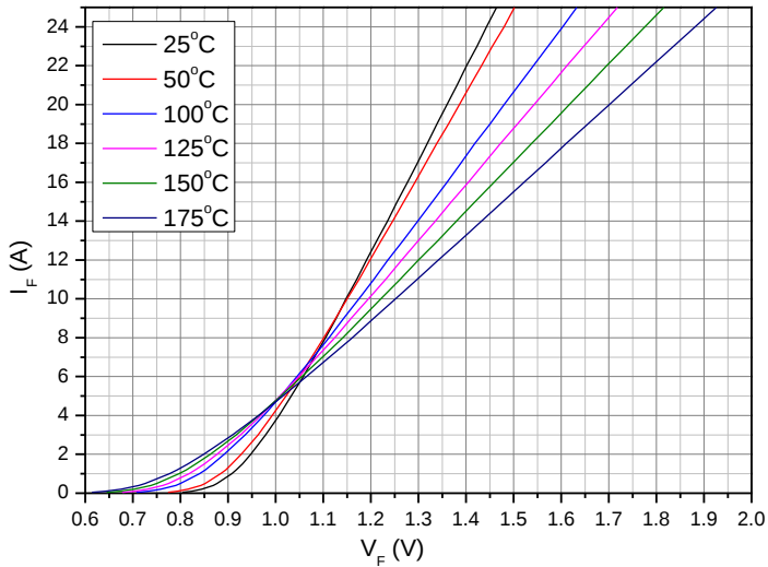
Figure 1. Forward Characteristics
