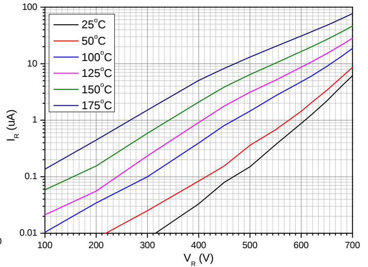
Figure 2. Reverse Characteristics
