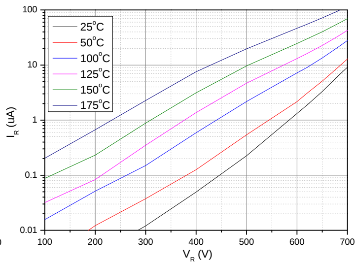
Figure 2. Reverse Characteristics
