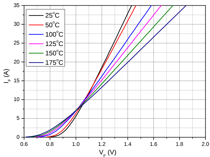
Figure 1. Forward Characteristics
