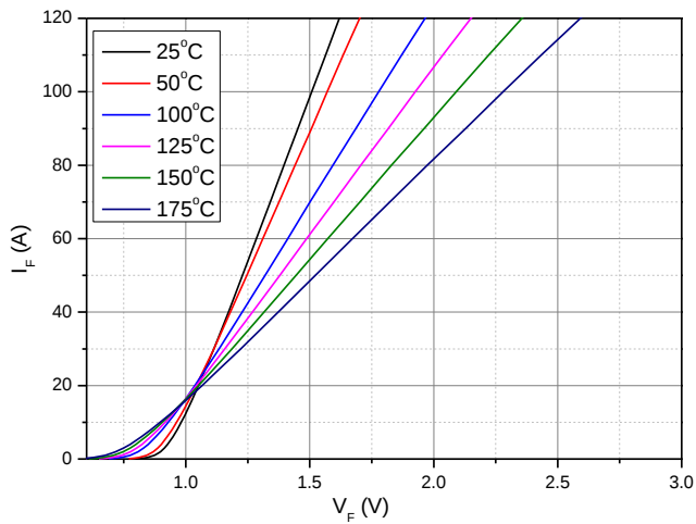
Figure 1. Forward Characteristics
