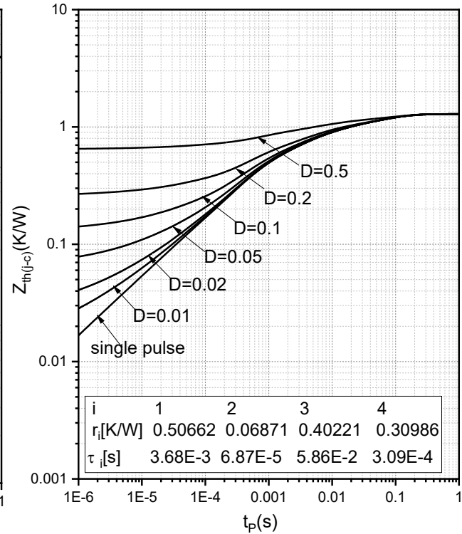
Fig.22 Transient Thermal Impedance (Diode)
