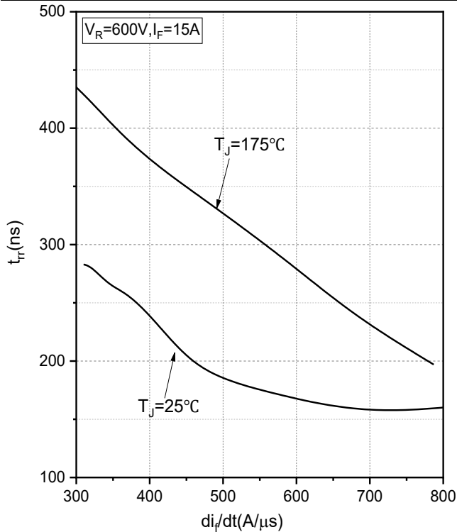
Fig.17 Typical Reverse Recovery Time as a Function of Diode Current Slope
