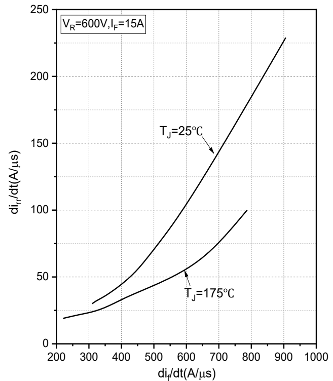
Fig.20 Typical Diode Peak Rate of Fall Of Reverse Recovery Current as a Function of Diode Current Slope
