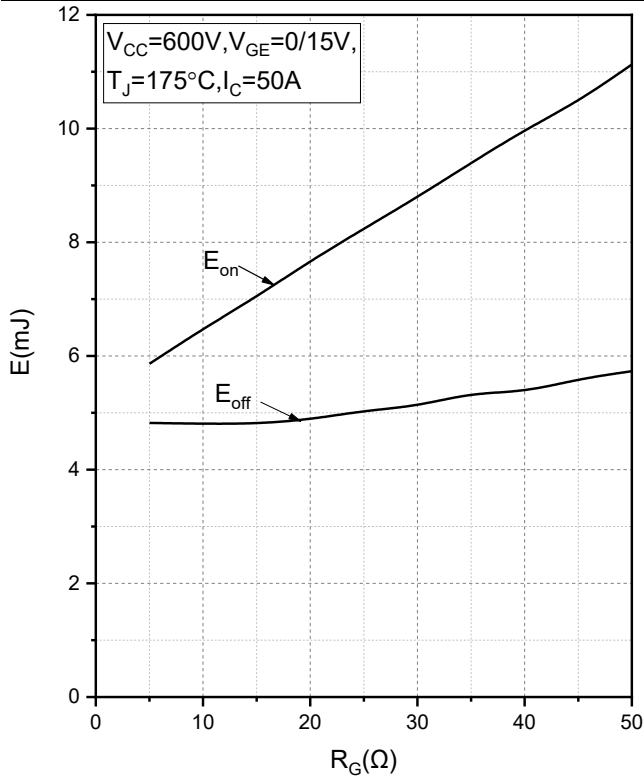
Fig.9 Typical Switching Energy Losses as a Function of Gate Resistor, T_J=175^\circ C
