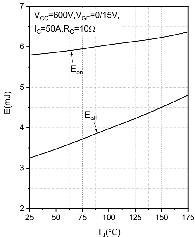
Fig.11 Typical Switching Energy Losses as a Function of Junction Temperature
