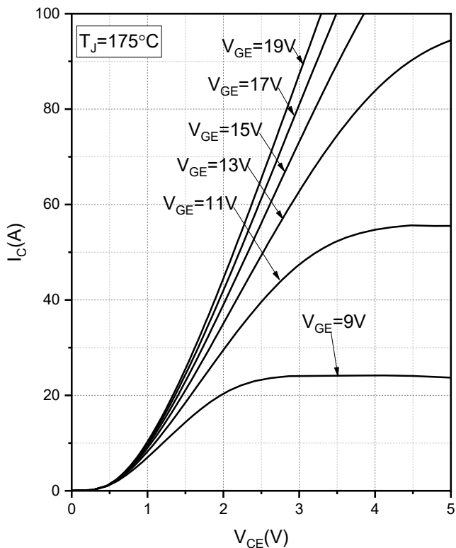
Fig.3 Typical Output Characteristics, T_J=175^{\circ}\text{C}
