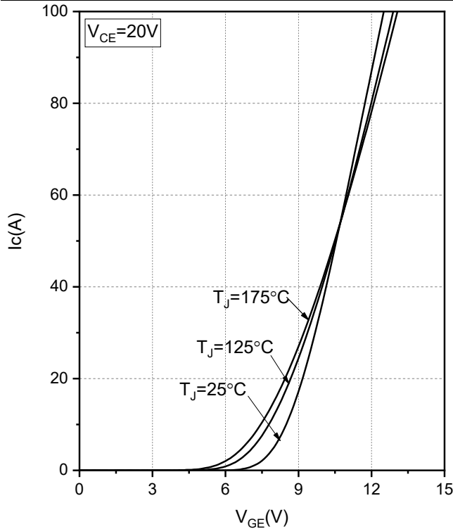
Fig.5 Transfer Characteristic
