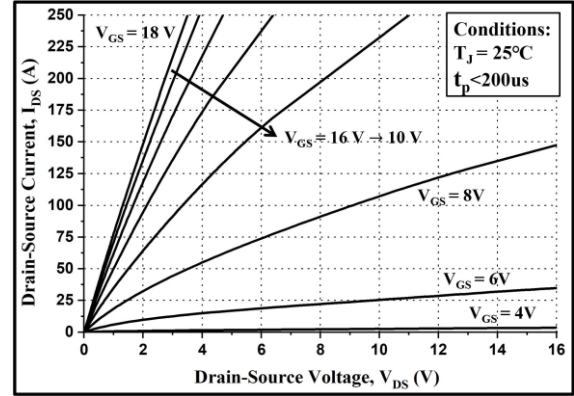
Figure 2. Output Characteristics T_J = 25^\circ\text{C}
