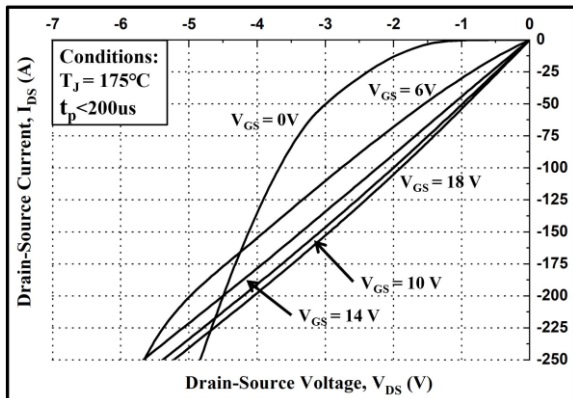
Figure 15. 3rd Quadrant Characteristic at 175^{\circ}\text{C}
