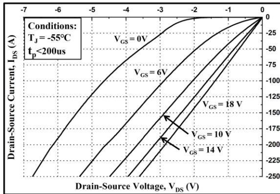
Figure 13. 3rd Quadrant Characteristic at -55^{\circ}\text{C}
