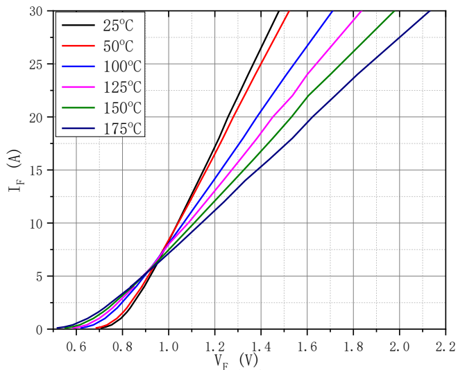
Figure 1. Forward Characteristics
