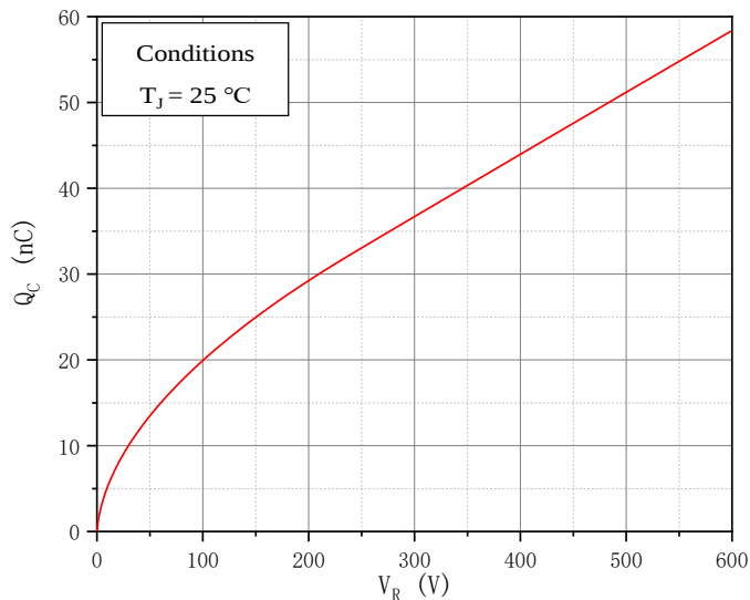
Figure 3. Total Capacitance Charge vs. Reverse Voltage
