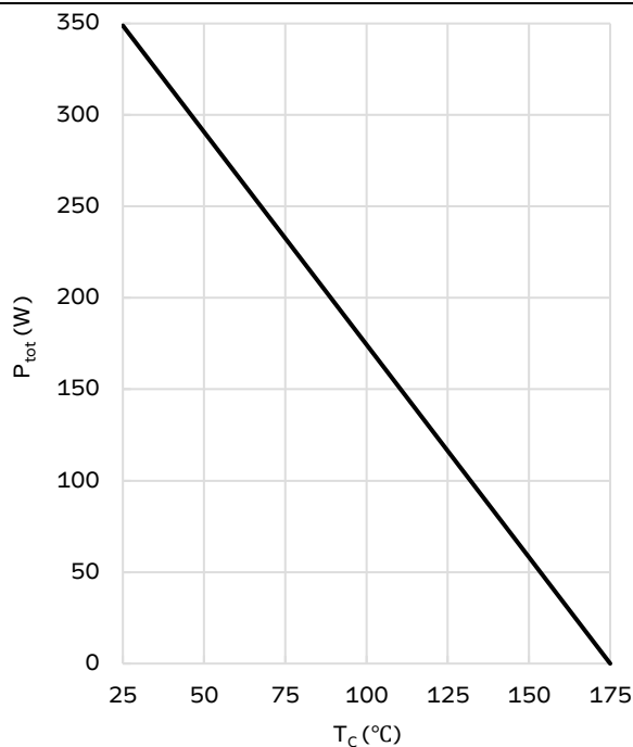
Figure 4. Power derating
