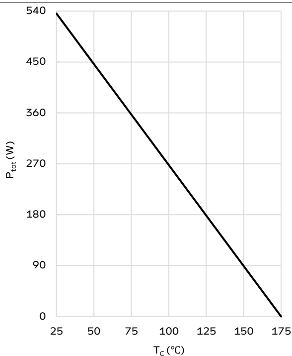
Figure 4. Power derating
