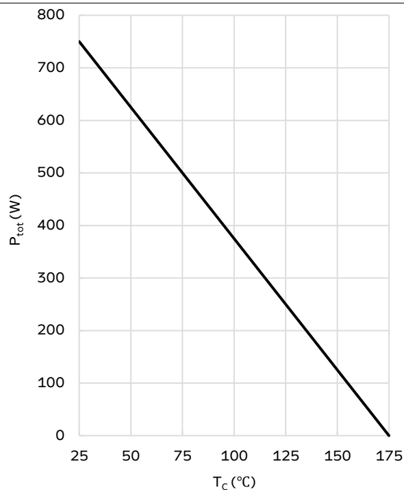
Figure 4. Power derating
