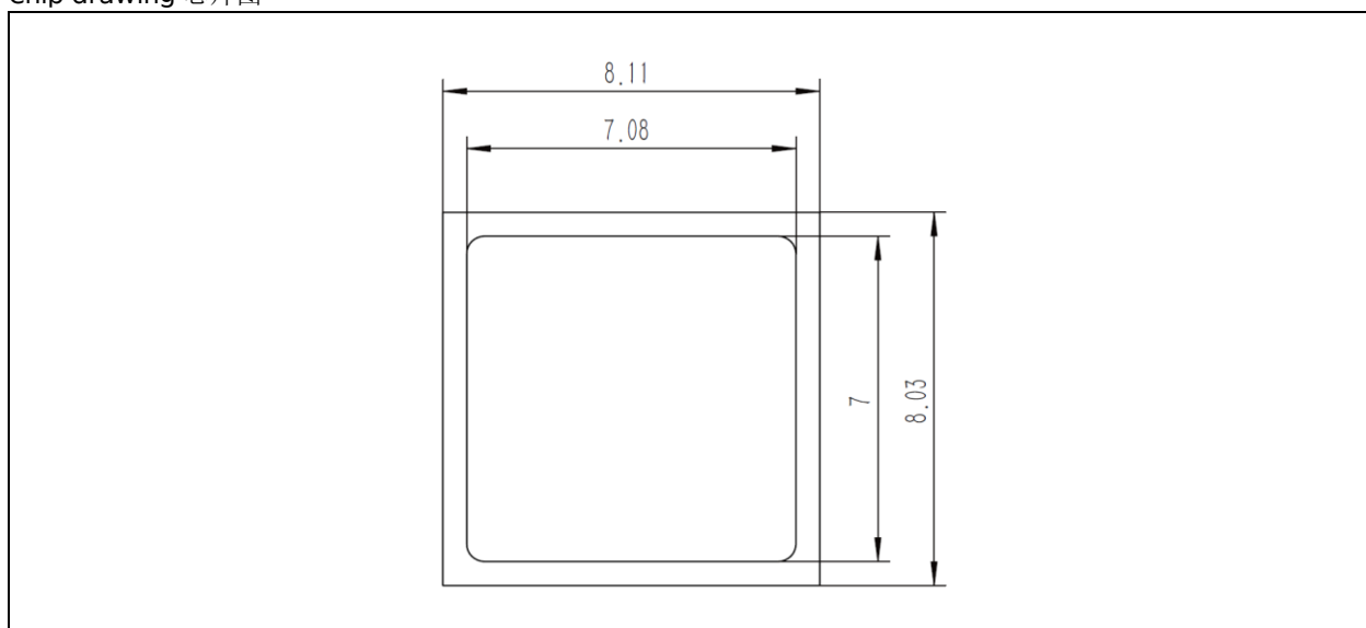
Chip drawing 芯片图
