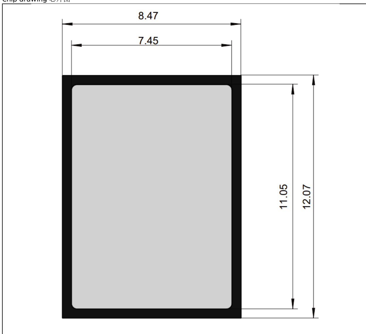
Chip drawing 芯片图
