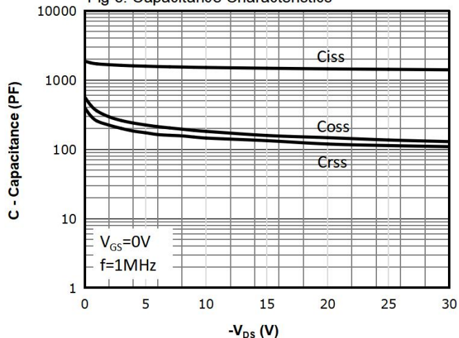
Fig 6: Capacitance Characteristics
