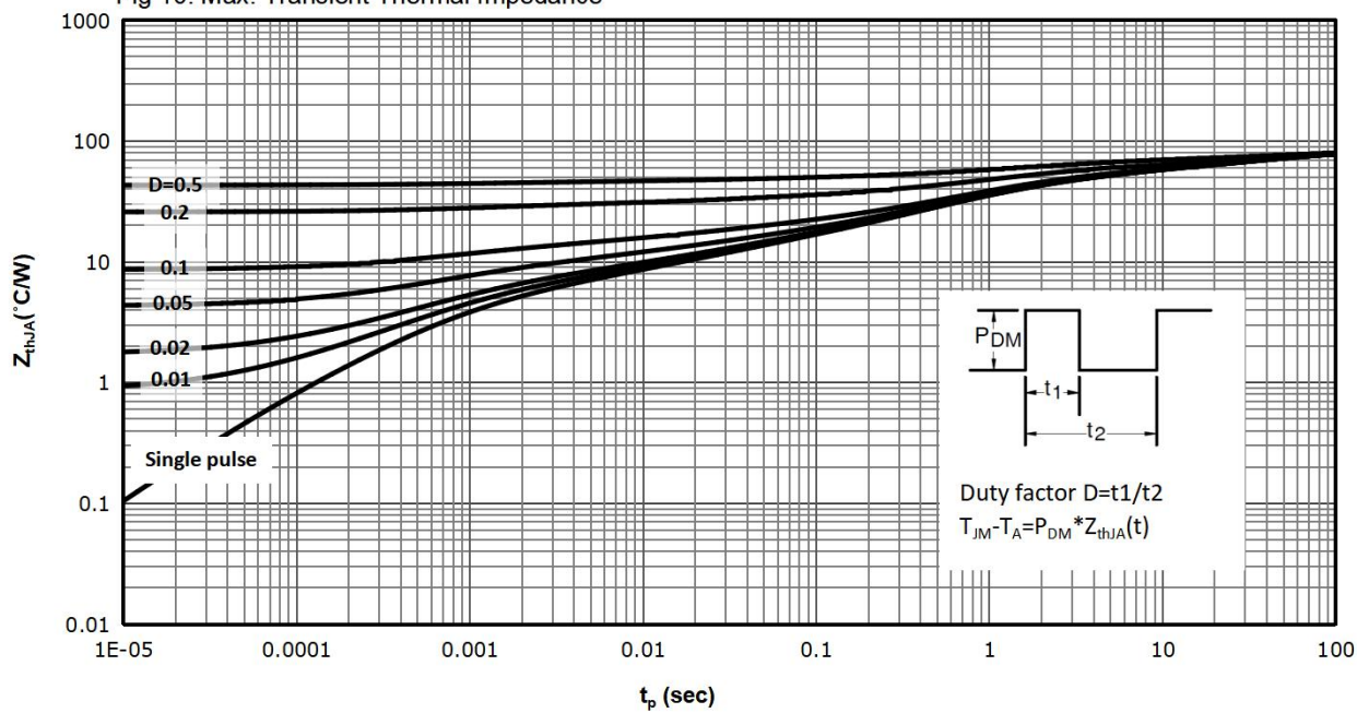
Fig 10: Max. Transient Thermal Impedance
