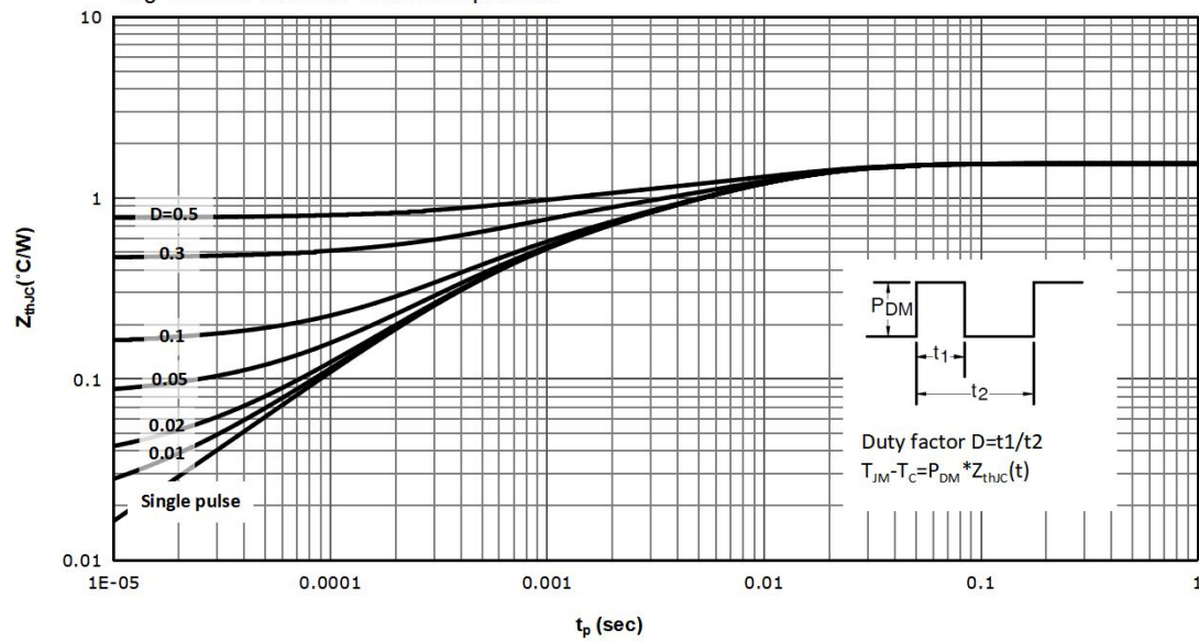
Fig 10: Max. Transient Thermal Impedance
