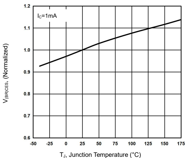
Figure 11 V_{(BR)CES} vs. Temperature
